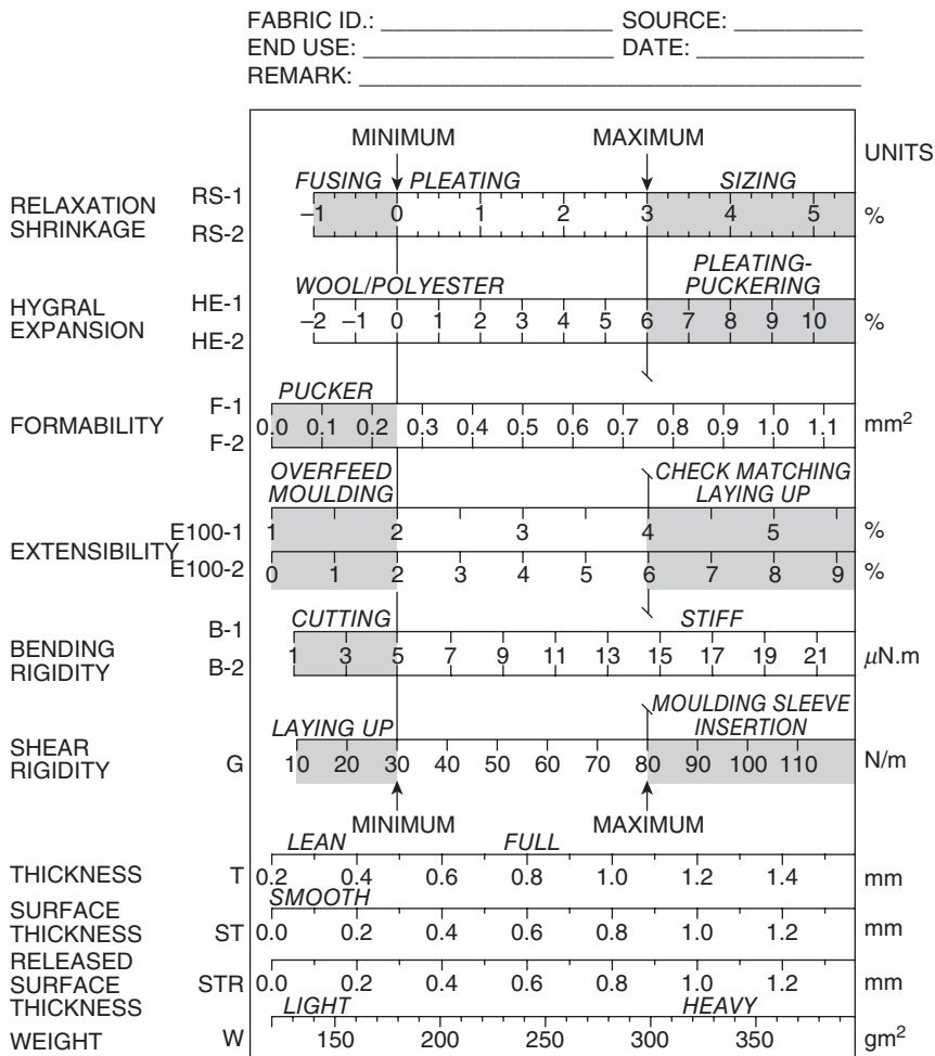
1.7 The FAST control chart for light-weight suiting fabrics. Source: Anon 64
